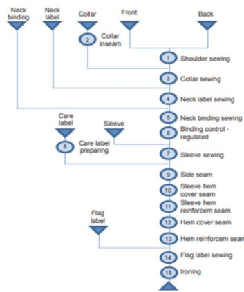
Figure 2. A Sample T-Shirt And Its Production Line
